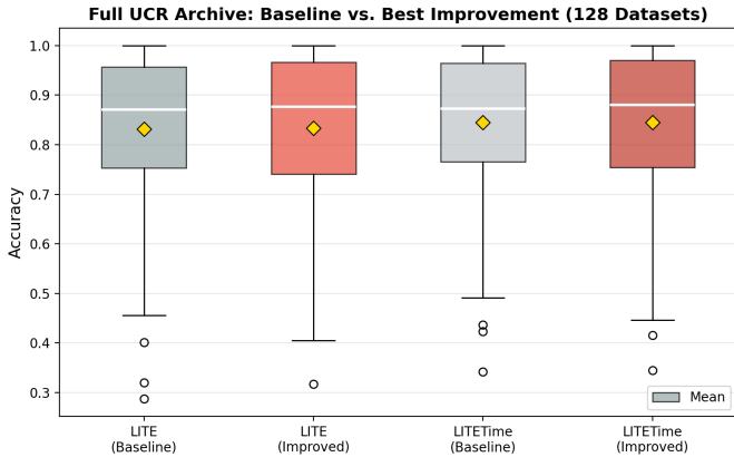
Fig. 9. Accuracy distribution comparison between baseline and improved configurations across the full 128-dataset UCR archive. The improved LITE configuration shows an upward-shifted distribution with a higher median, while LITETime performance remains essentially unchanged. Gold diamonds indicate mean accuracy values.
